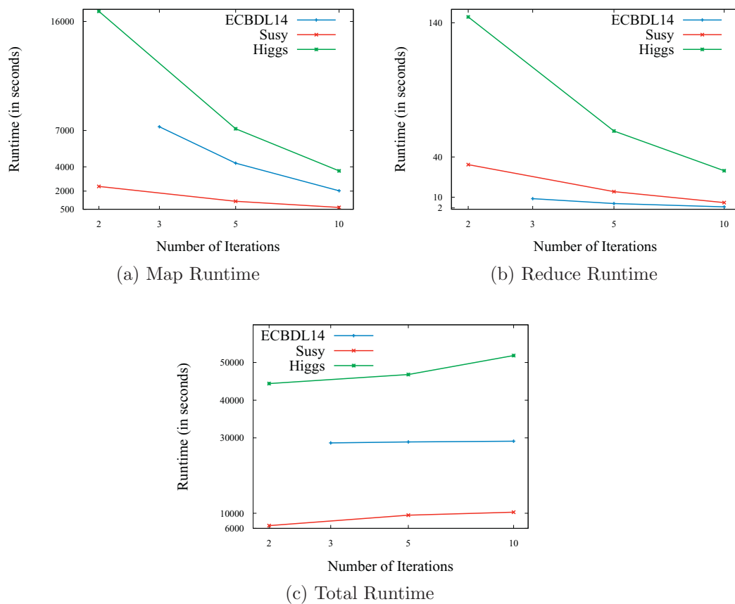
Fig. 11. Runtimes vs number of iterations.
