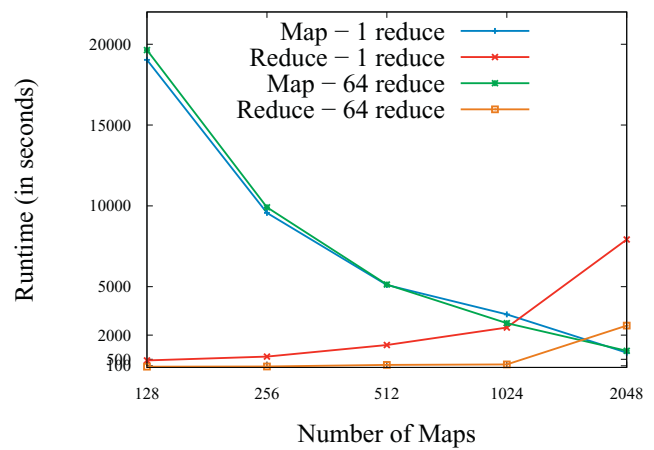
Fig. 9. Map and Reduce runtimes required according to the number of maps - HIGGS.
